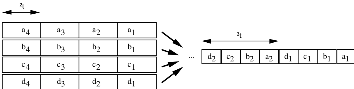
Figura 2-13: TDM
