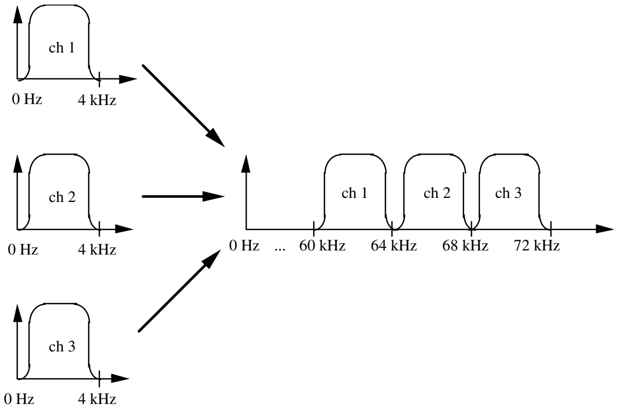
Figura 2-12: FDM
